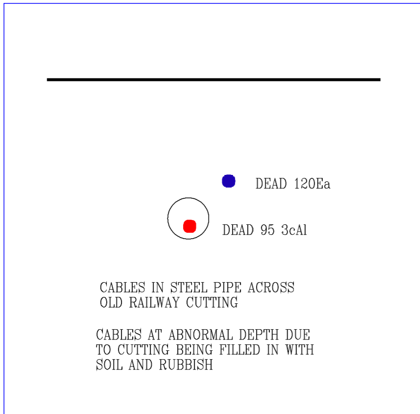
Cross Section (2520669)
