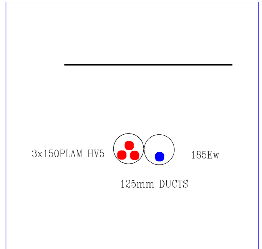
Cross Section (2898461)
